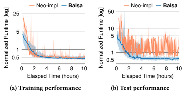
Figure 15: Comparison with learning from expert demonstrations.
