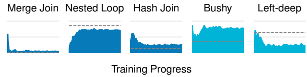
Figure 18: Balsa’s use of join operators (dark blue) and plan shapes (light blue) on JOB. Dashed lines are counts from PostgreSQL plans.
