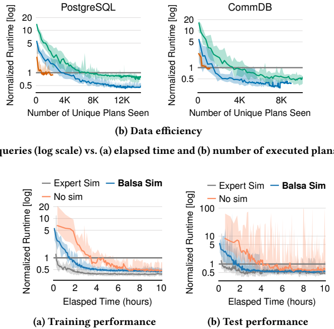
Figure 10: Impact of the initial simulator. (a) Better simulators accelerate learning. (b) Simulation is essential for generalization.
