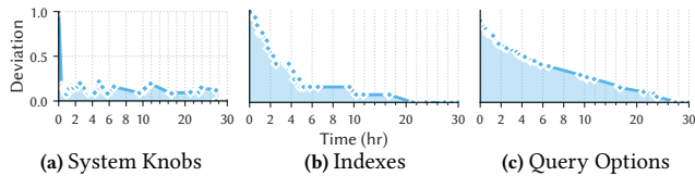
Figure 8: Configuration Time Analysis – Normalized deviation from the final configuration over time for 12 resource-related system knobs, indexes, and query options using Proto-X’s best JOB trial. A configuration’s deviation is the average difference of values from the final configuration.
