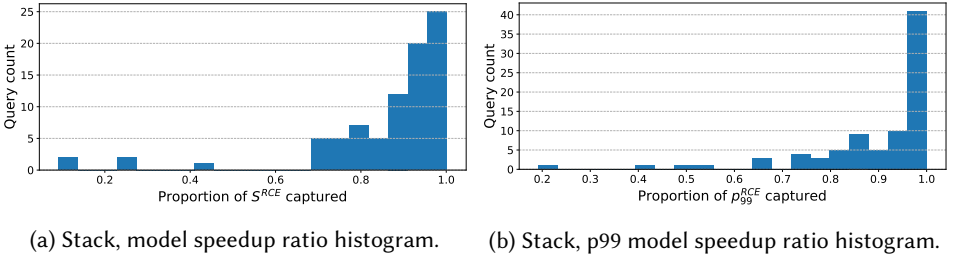
Fig. 8. Model results on Stack.
